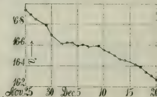
FIG. 24.—Chart showing loss of standard volumes of gas in diver in lapse of days. Diffusion of air through KCl solution.
